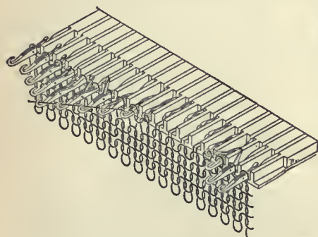
FIG. 9.—Individual Action of the Latch Needle.
